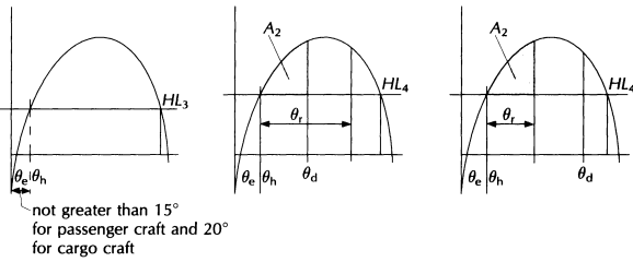
Figure 2 – Damage stability
