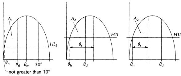
Figure 1 – Intact stability
